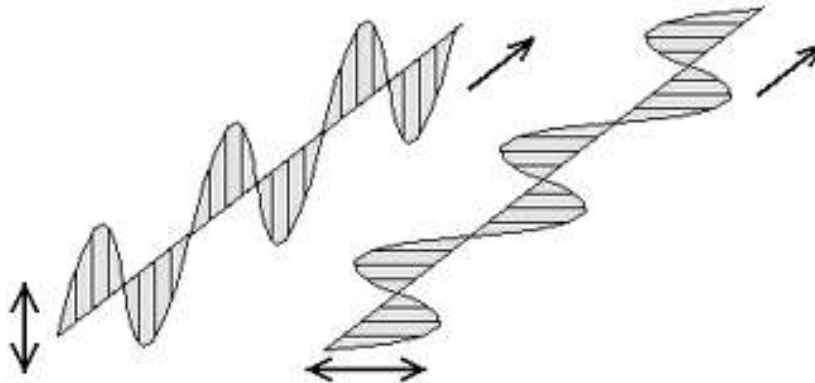
Fig.3: Diagram showing vertically and horizontally polarised light
