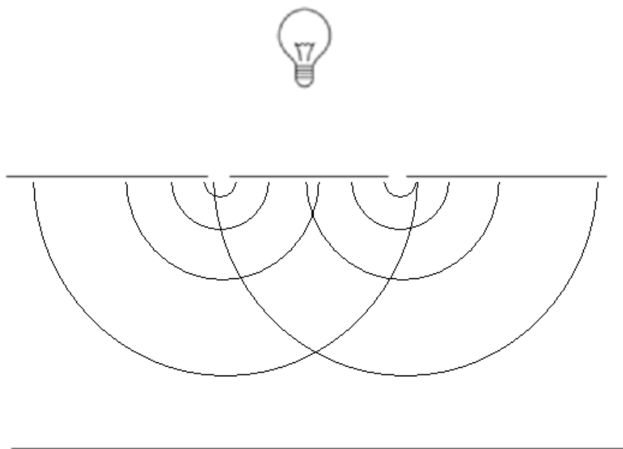
Fig.1: Light waves in the twin slit interference experiment
