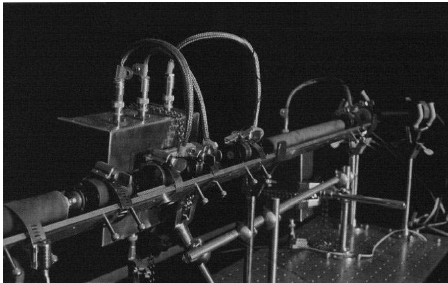
Fig.4: Quantum cryptographic apparatus constructed at IBM. Flashes of polarised light, each one tenth of a photon, are generated and measured across a free air optical path of 32 centimetres.
